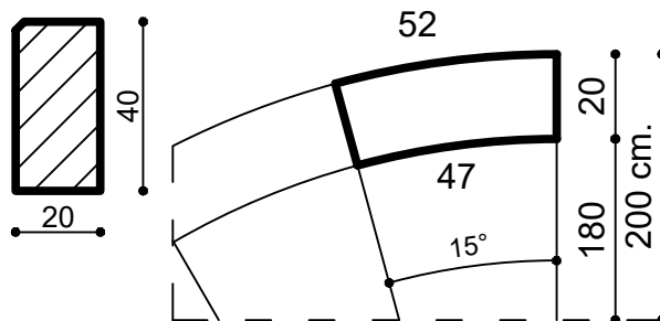
SEZ 20x40 cm Re = 2,0 mt
