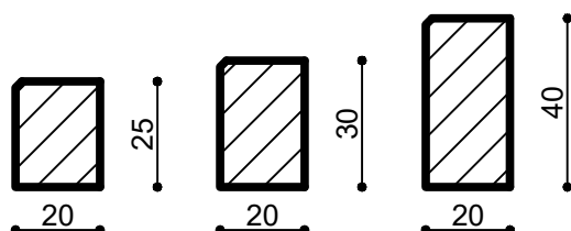
SEZ 20x25 , 20x30 e 20x40 cm Re = 1,0 mt
